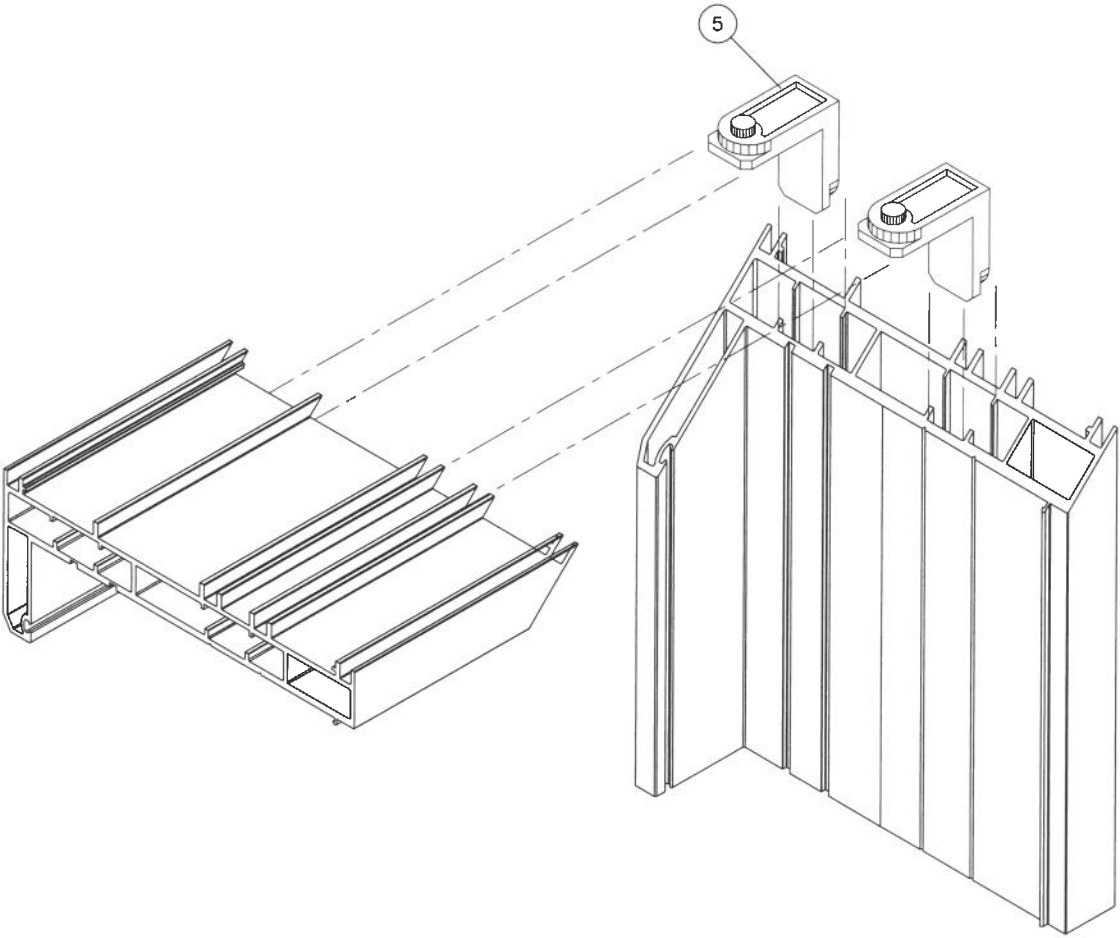
FRAME CORNER
